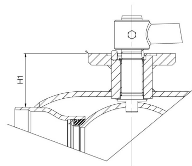
DN 200-250
