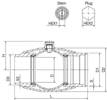
DN 150
