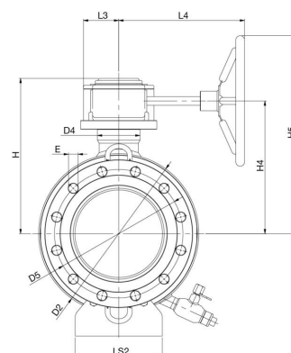
DN 150-900
